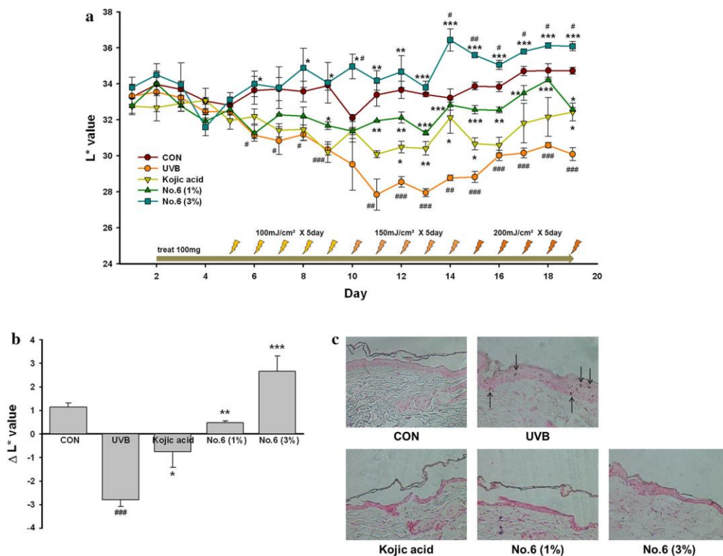
Figure 10. Effects of aerial part of P. thunbergiana on pigmentation in UV-irradiated animal. a Melanin possessing hairless mice were treated with 100 mg of cream base, kojic acid 1 % cream, No. 6 1 and 3 % cream on dorsal skins every day. UVB irradiation was performed according to the indicated schedules. The lightness ( L^* value) of skin was measured before applying cream on each day. b \Delta L^* values of each animal were calculated; values of days 17, 18, 19 minus values of days 2, 3, 4. Data represent mean \pm SEM (n = 3). #p<0.05, ##p<0.01, and ###p<0.001 compared with CON. *p<0.05, **p<0.01, and ***p<0.001 compared with UVB group. c Microscopic images of skin sections. Melanogenesis of dorsal skin was highlighted by Fontana–Masson staining. Arrows indicate pigmentation)
