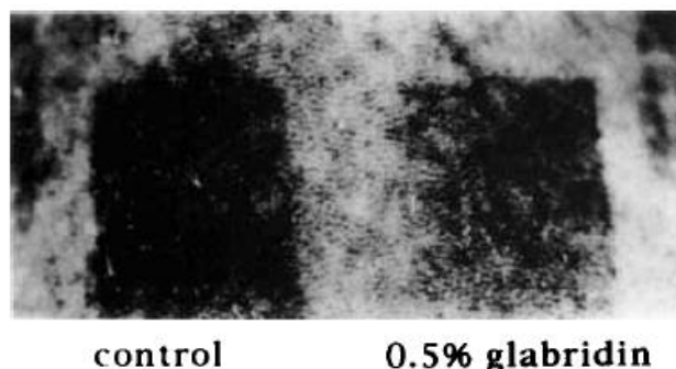
Figure 4. Effect of glabridin applications on UVB-induced pigmentation in the back of a brownish guinea pig. Two pigmented square-shaped areas were exposed to UVB irradiation (250 mJ/cm 2 /day for four successive days), and then, 0.5% glabridin (or base solutions for the control) were topically applied for 3 weeks. Reduced pigmentation was seen in glabridin-treated skin. Similar results were obtained on all three guinea pigs tested.
