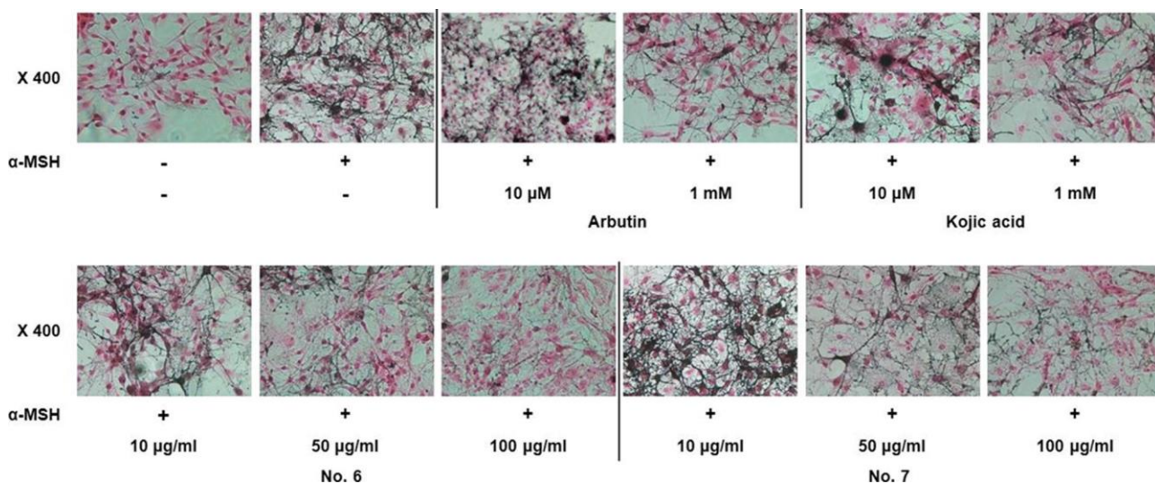
Figure 8. Optical images (magnification 9400) showing melanin content with Fontana–Masson staining in B16F10 cells. After 24 h of \alpha -MSH pre-incubation, B16F10 cells were treated with a combination of \alpha -MSH and extract No. 6 or 7, arbutin, or kojic acid for 48 h. Pigmentation observed upon Fontana–Masson staining (magnification x 400)
